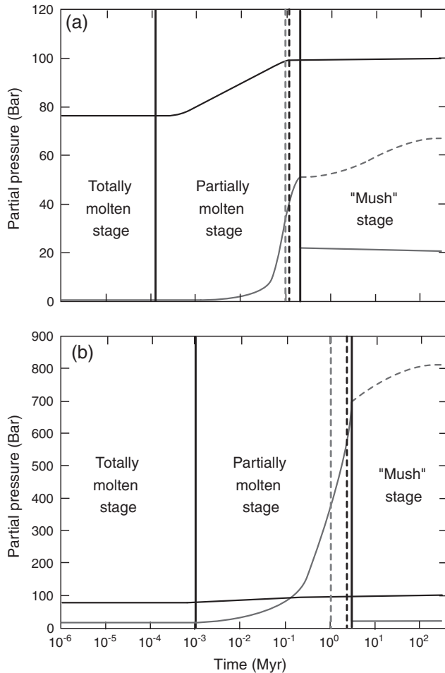
Figure 5. Time evolution of partial pressure of uncondensed H 2 O (grey line), total H 2 O (condensed and uncondensed) (grey dashed line) and CO 2 (black line) for an initial amount of H 2 O of (a) 1.4 \times 10^{-2} wt % and (b) 1.4 \times 10^{-1} wt %. The mass fraction of dissolved CO 2 is constant and equal to 1.4 \times 10^{-2} wt %. Condensation of water vapor occurs at the end of the magma ocean phase ( t_c = t_p ). It corresponds to the beginning of the mush stage shown by the vertical lines on the figure. For comparison, we also draw a dashed line corresponding to a threshold of 98% solidification in volume (grey line) [Elkins-Tanton, 2008]. Parameters used for the calculations are given in Table 4.
