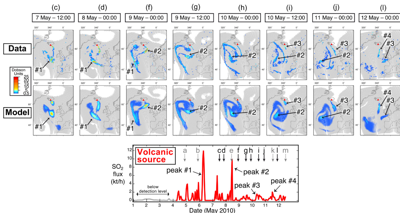
Fig. 5. Comparison of observed and modelled atmospheric evolution of the Eyjafjallajökull plume in May 2010. Data: maps of SO 2 column amounts (CA in DU) derived from the processing of IASI satellite observations acquired over a 12 h time window, centred on the date indicated above. Model: maps of SO 2 CA simulated with CHIMERE chemistry-transport model, using the source reconstructed by multiple-image inversion (bottom plot). Regions in grey indicate column amounts less than 0.5 DU, which corresponds to the detection threshold in IASI processing (see Sect. 2.2 for details). Source: time series of the SO 2 flux (kt h -1 ) retrieved from the inversion procedure using the 13 IASI images available for the period from 1 to 12 May 2010 (numbered (a) to (m) and indicated with arrows). The complete time series of observed and modelled maps is available in the Appendix (Figs. A1 and A2). As illustrated by a few examples, peaks in the SO 2 flux create dense puffs in the plume which can be tracked up to 6 days after their emission.
