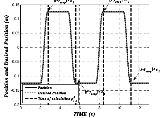
Fig. 8.a : Position & Desired Position (m)
