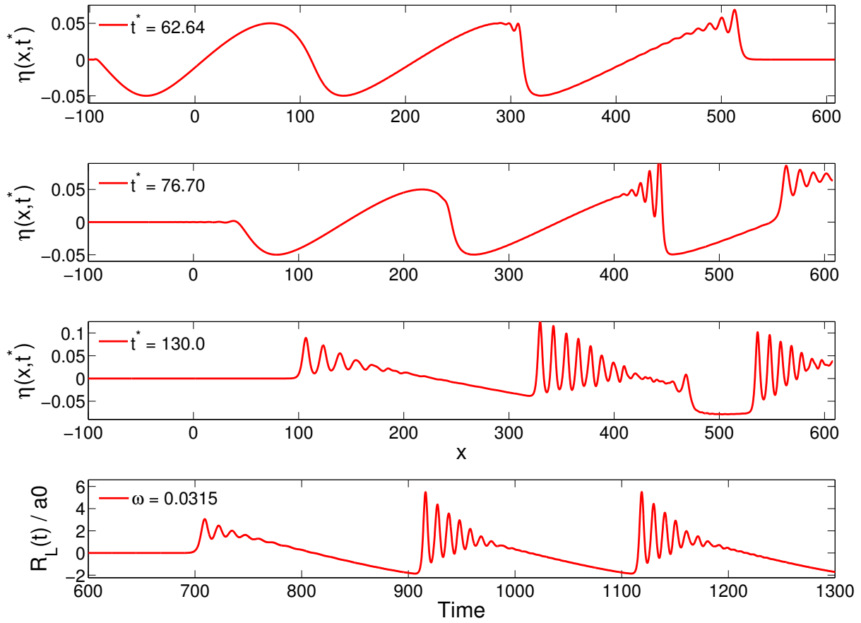
Figure 5. Time evolution of the free surface elevation as a function of space, at three different times t^* (first three top panels) reported on the figure. The figure refers to the three-wave case with frequency \omega = 0.0315 . The lower panel reports the maximal elevation at the wall R_L/a_0 as a function of time.
