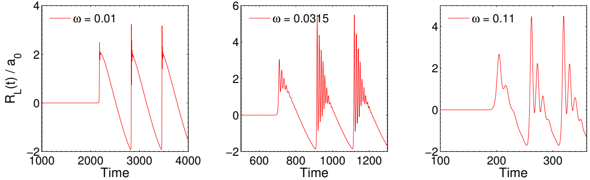
Figure 7. Time evolution of the wave run-up on the vertical wall for the three incident wave case recorded for several values of the incoming frequency \omega . The maximum run-up is achieved for \omega_{\max} \approx 0.0315 .
