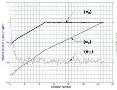
Fig. 12. Evolution of displacement error: xy\alpha robot
