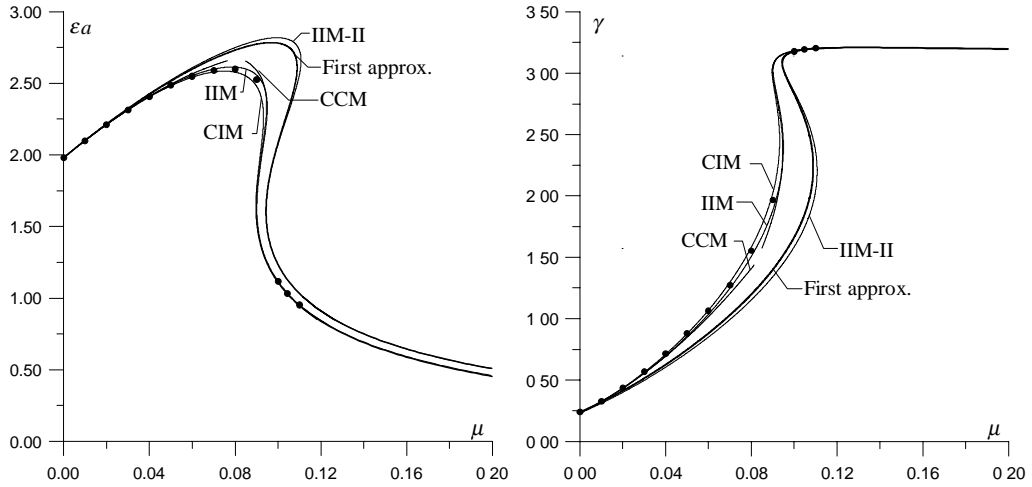
Figure 3. Amplitude and phase response vs. detuning in the second approximation; ● numerical results.
