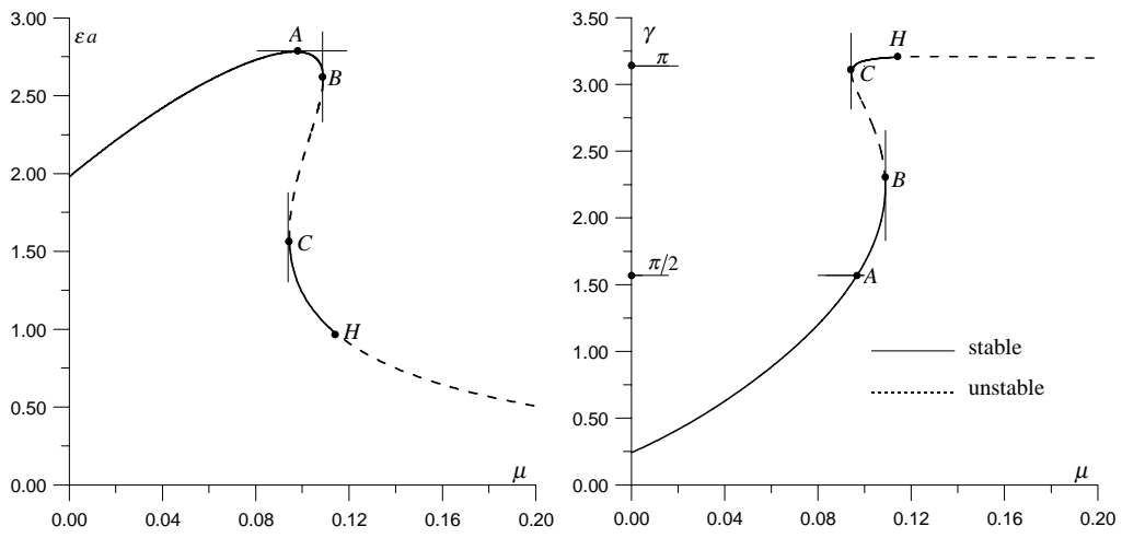
Figure 2. Amplitude and phase response vs. detuning in the first approximation.
