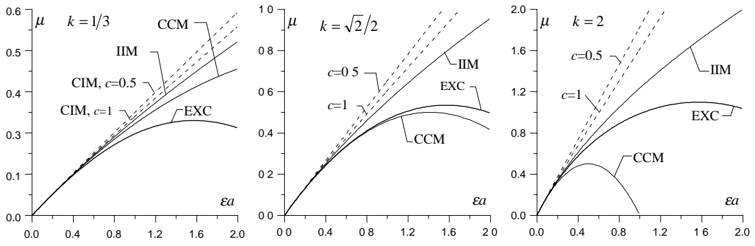
Figure 1. Equilibrium paths for the one-d.o.f. sample system.
