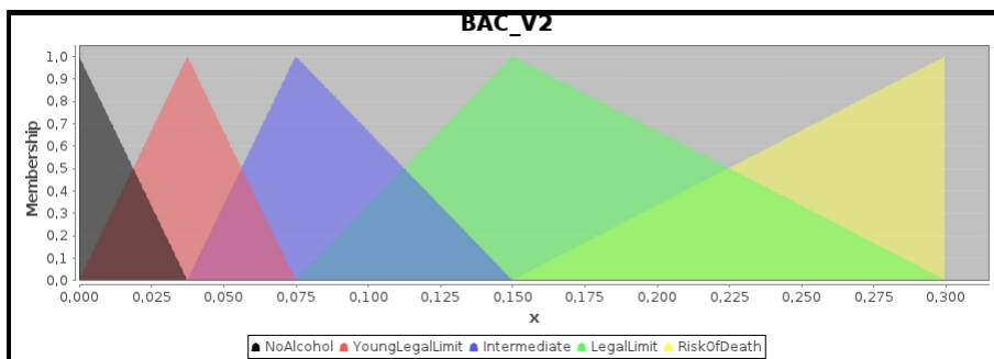
Fig. 3. Fuzzy partition generated by Herrera & Martínez' approach.
