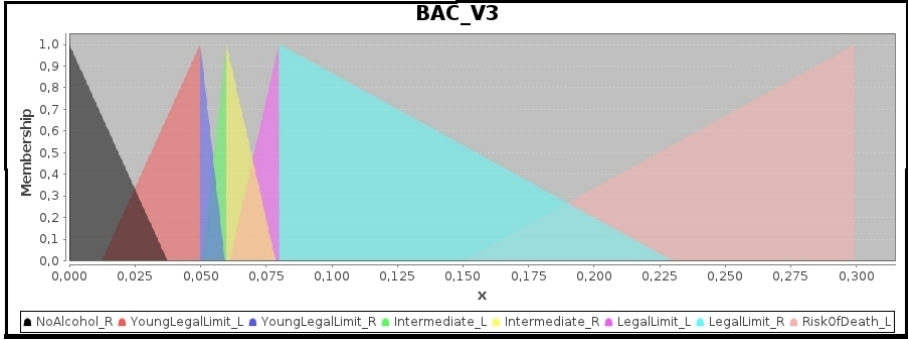
Fig. 4. Fuzzy partition generated by our algorithm for the BAC example.
