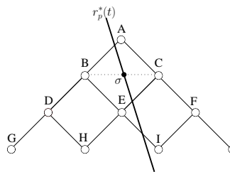
Figure 2. Fourth order scheme.
