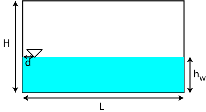
Figure 12: Tank partially filled up with water submitted to an horizontal excitation. Here, the dimension of the box is: L = 1.73 m, H = 1.15 m, and the tank is filled up with a height h_w of water. N_x = 173 and N_y = 115 . We measure the evolution in time of the height of the water at d = 0.05 m of the left border of the tank.
