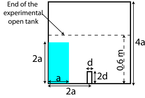
Figure 5: Collapse of a water column with an obstacle. The initial gate which retains the column of water disappears at the initial time and the column of water collapses. The parameters are a = 0.25 m and d = 0.04 m.
