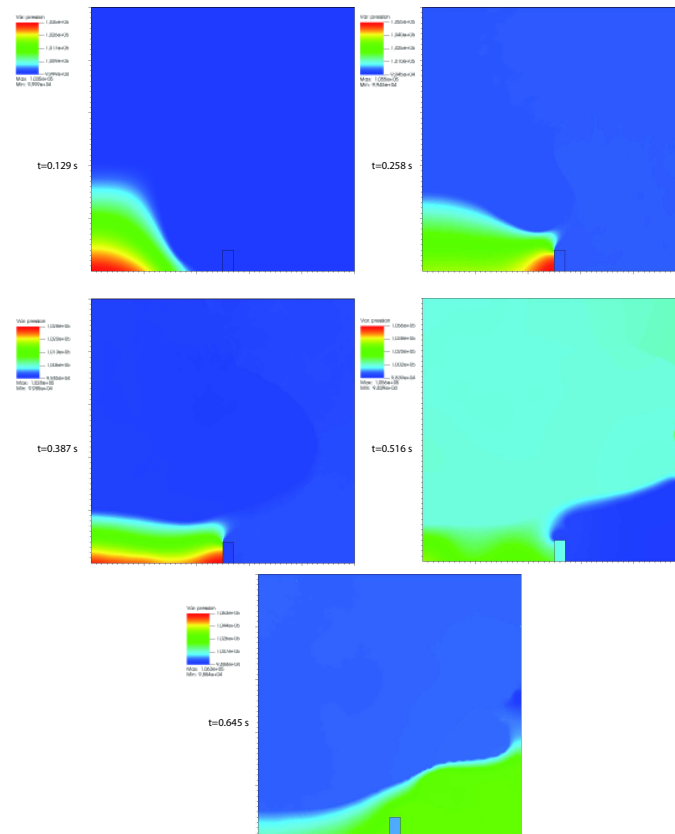
Figure 11: Dam Break test case with an obstacle with the ODYSSEY code. We show the pressure field. In particular, at t = 0.258 s and t = 0.387 s, we see a pressure peak due to the obstacle at the middle of the box.
