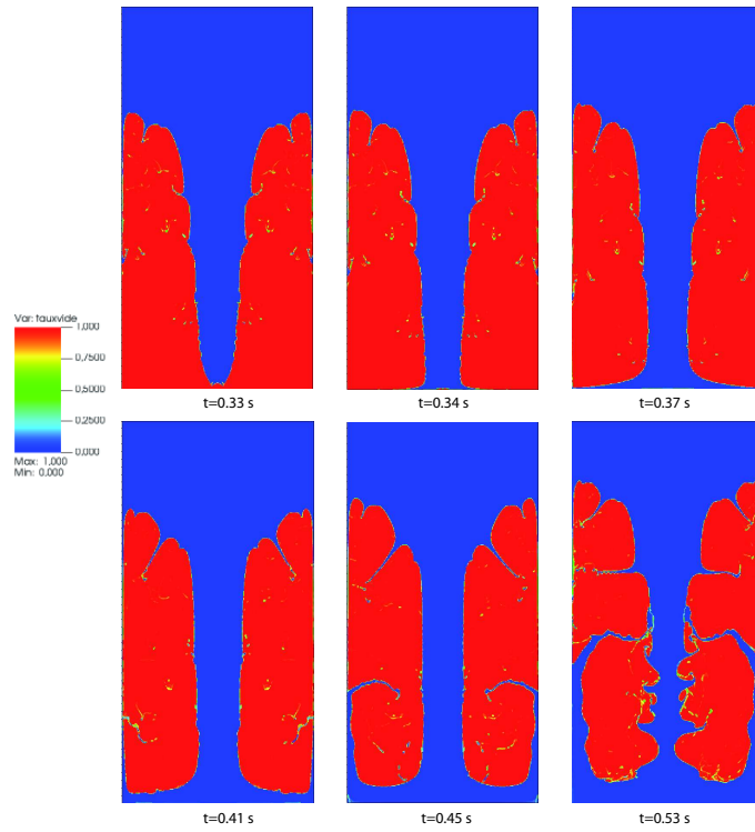
Figure 21: Rayleigh-Taylor instabilities. Development of a main needle followed by secondary fine needles and topology changes. The overall symmetry of the computational is globally fulfilled.
