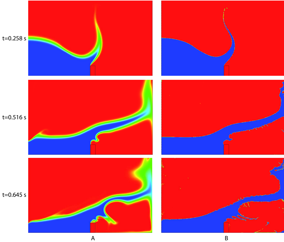
Figure 8: Accuracy of interface capturing. A first order projection (case A ) is compared to the (also first order but) low-diffusive procedure (case B ). It is observed that numerical diffusion is mainly suppressed and complex interface details can be tracked.
