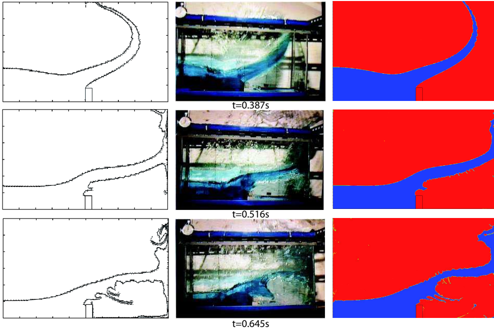
Figure 7: Collapse of a water column with an obstacle at longer time. The results are in agreement with the experiments and the other simulation. In particular, in the next snapshots ( t = 0.645 s), our code developed the same patterns near the obstacle and a gas pocket on the top right corner, similarly to the experiment.
