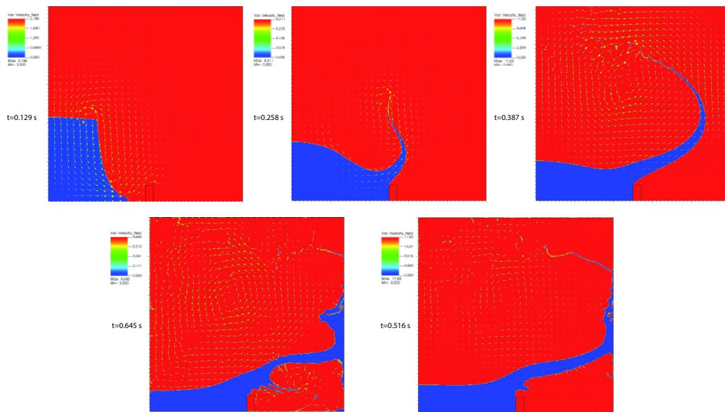
Figure 10: Dam Break test case with an obstacle with the ODYSSEY code. We superimpose both gas volume fraction and velocity field. Thanks to the representation of this vector field, we better understand the motion of the free surface flow.
