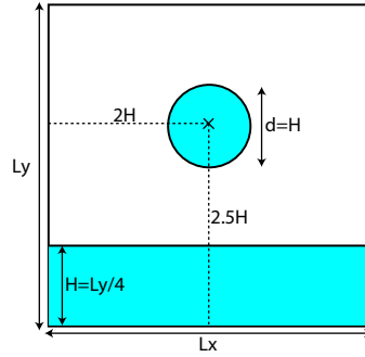
Figure 16: Free fall of water and impact with water at rest. The box size is: Lx = Ly = 0.584 m ( Nx = Ny = 350 ). The height of the water layer is H = Ly/4 = 0.146 m and the radius of the water disk is H/2 = 0.073 m, put at the middle of the box and at 2.5H from the bottom of the box.
