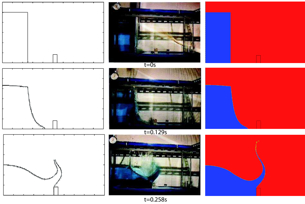
Figure 6: Collapse of a water column with an obstacle. At left, the results obtained with the code of Greaves, in the middle, the results of Koshizuka et al. and at right the results with our code ODYSSEY. Small deviations at the beginning between numerical and physical experiments originate from the finite time necessary for the removal of the gate. Otherwise, it is essentially in good agreement with referred results.
