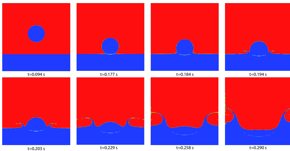
Figure 17: Free fall of a disk of water and impact with water at rest. Evolution of the volume fraction of gas \alpha at different time steps. The smashing of the sphere conducts to the formation of two jets on either side of the initial disk.
