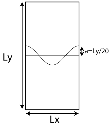
Figure 19: Configuration: Lx = 0.5 m, Ly = 1 m, Nx = 300 , Ny = 600 . The border between air and liquid is disturbed at a height of Ly/2 by a sine-shaped signal: Ly/2 + Ly/20 \cos(2\pi x/Lx) .
