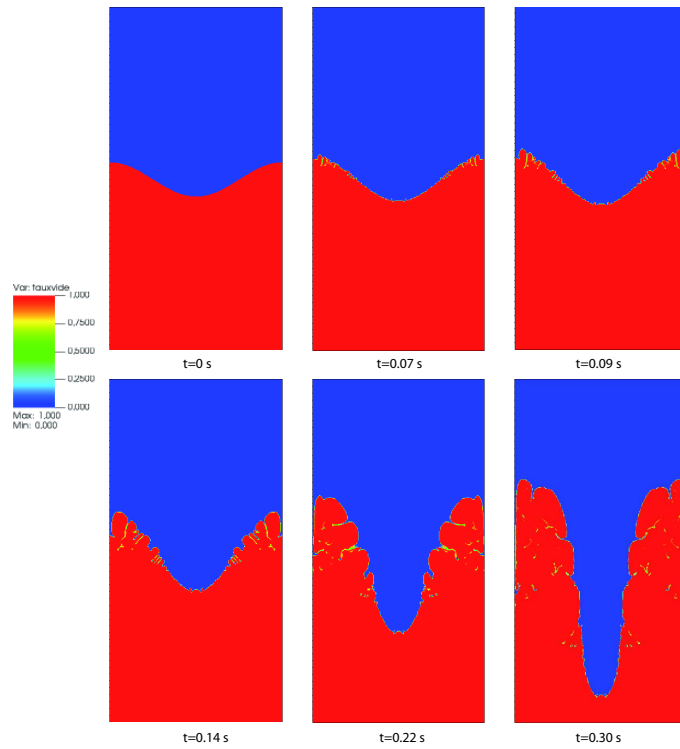
Figure 20: Rayleigh-Taylor instabilities. Heavy (water) fluid above the light one (gas) with a sine-shaped perturbation of the initial interface.
