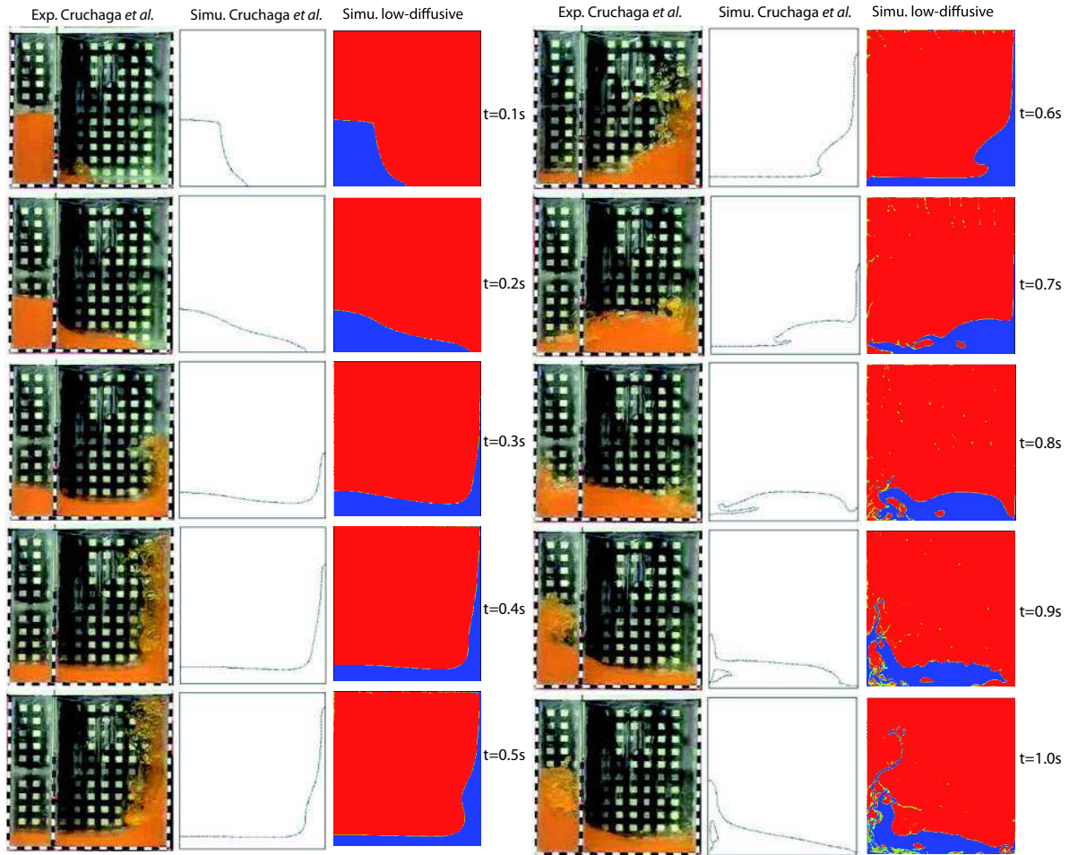
Figure 3: Collapse of a column of water. The experimental (resp. numerical) results of Cruchaga et al. (2007) are at left (resp. in the middle) and the results with our code ODYSSEY at right are compared at different time step. Except at the initial time where we see that the rise of the gate has a little impact on the experiment (not taken into account by the codes), the collapse of the column with our code gives results in very good agreements with those of Cruchaga et al. . Up to the time t = 0.6 s, the numerical results are indeed very similar. In the next snapshots, discrepancies are mainly due to the droplets which fall from the upper wall (in particular at the left bottom of the box), which is not the case in the simulation of Cruchaga et al. since they have taken open boundary conditions for the upper wall.
