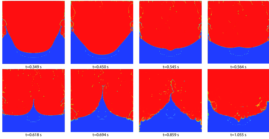
Figure 18: Free fall of a disk of water and impact with water at rest. Evolution of the volume fraction of gas \alpha at longer time step. The gap generated by the fall of the disk is progressively filled up due to the falling of the jet of water at right and left of the box due to the gravity. This motion conducts at the end of the presented snapshots to the formation of a new bouncing jet at the middle of the box due to the meeting of the two lateral ones. The expected symmetry is well-conserved during quite a long time.
