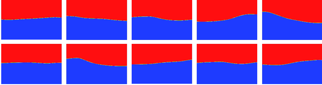
Figure 13: Tank partially filled up with water submitted to an horizontal excitation, with h_w = 0.6 m and a period for the tank of T = 1.3 s. We represent the volume fraction of the gas (always gas in red and water in blue) at different times: t_1 = 0.52 s, t_2 = 0.92 s, t_3 = 1.32 s, t_4 = 1.72 s, t_5 = 2.52 s for the first line and t_6 = 2.92 s, t_7 = 3.92 s, t_8 = 4.92 s, t_9 = 6.52 s, t_{10} = 7.12 s for the second line. Due to the horizontal excitation of the tank, a wave initiates and displaces from left to right and right to left with an amplitude which increase up to t \simeq 3.5 s before decreasing and having a situation more stable at t = 6.54 s. After, the amplitude of the oscillation increases again ( cf. Fig. 14).
