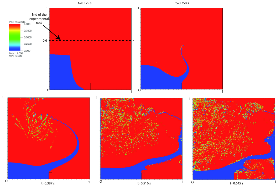
Figure 9: Collapse of a water column with an obstacle. Snapshots of the concentration of gas c_g . We represent the whole numerical box (without the cut at h = 0.6 m). After the formation of a wrapped motion, we observe some numerical diffusion due to the ejection of droplets initiated from the edge of the wave. Outside of this zone, the diffusion of the interface of the free surface flow is restricted to one cell. At the final time ( t = 0.645 s), these small amount of liquid begin to slightly disturb the free surface on the bottom right due to the fall of droplets due to gravity. But this diffusion appears only in terms of mass and not in term of volume of water which remains negligible.
