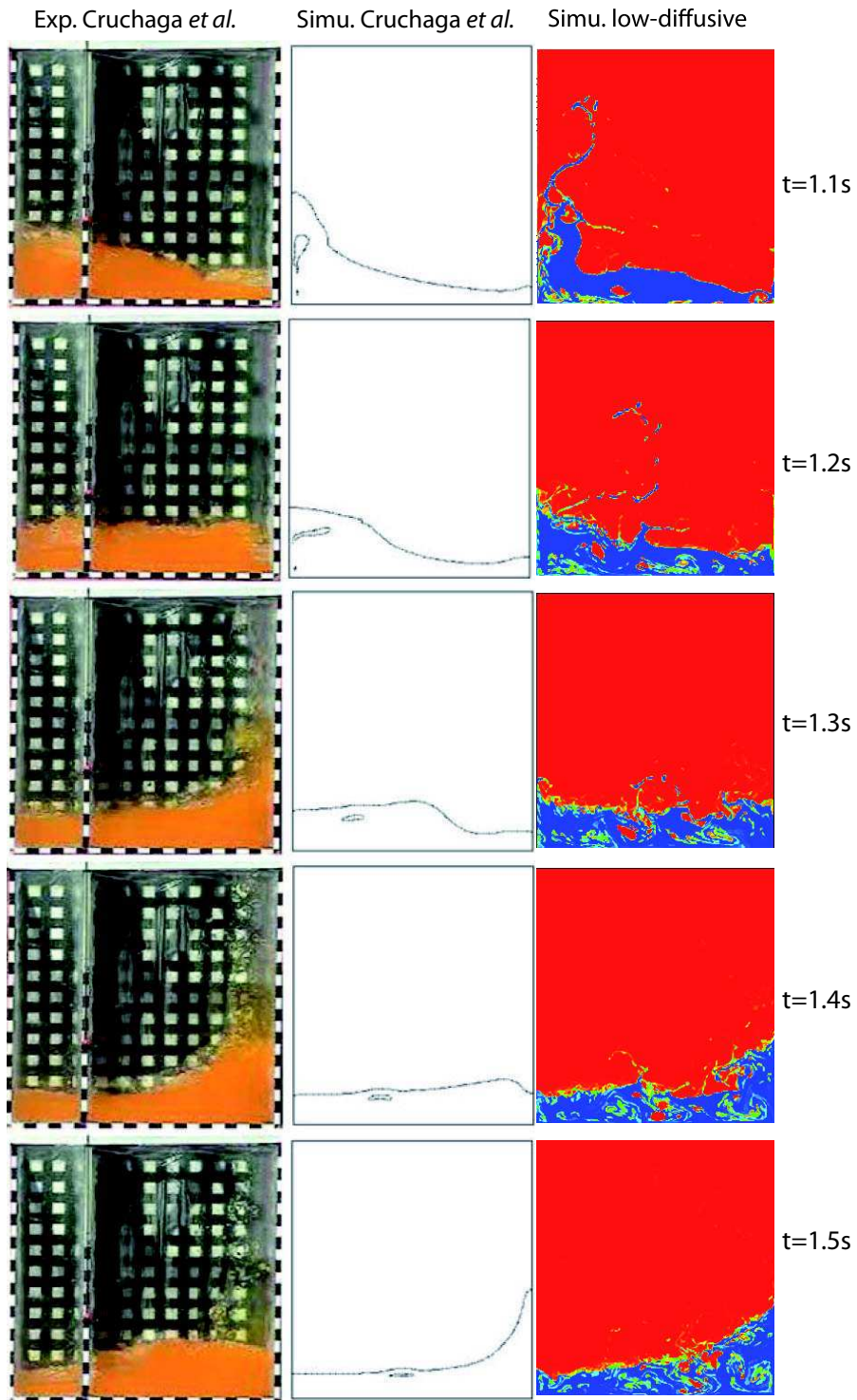
Figure 4: Same as Fig. 3 at longer time. At these times (especially the three last shots), our code reproduces better the experiment than the numerical code of Cruchaga et al. . The evolution in time of the water is well reproduced by our code, the agitation we still observe is due to the fact that our model does not take into account viscosity.
