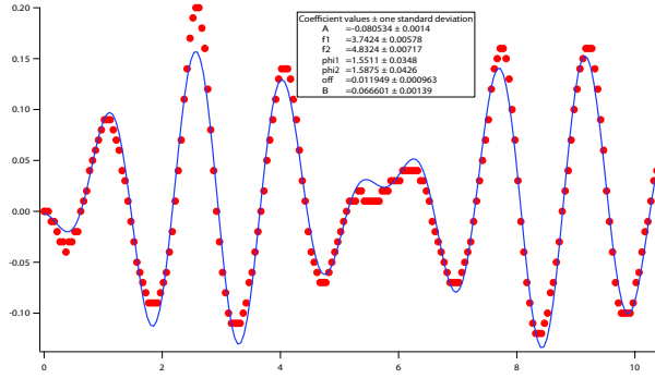
Figure 15: Fit of the curve representing the evolution in time of the free surface elevation of the water given by our code with a function f(t) : f(t) = A \sin(\omega_1 t + \phi_1) + B \sin(\omega_2 t + \phi_2) (curve given by our code in dotted red line and fitted curve in plain blue line). We obtain for the two frequencies: \omega_1 = 3.74 rad/s and \omega_2 = 4.83 rad/s. The first one is very closed to the natural frequency of the fluid ( \omega_{\text{fluid}} = 3.77 rad/s) and the second to the induced frequency of the box ( \omega_{\text{forced}} = \frac{2\pi}{T} = 4.83 rad/s).
