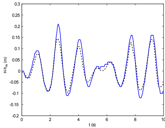
Figure 14: Tank partially filled up with water submitted to an horizontal excitation, with h_w = 0.6 m and a period for the tank of T = 1.3 s. We represent the free surface elevation, i.e. the height of the water relatively to the initial height h_w . We superimpose to our results (plain blue line) the scanned experimental curve of Faltinsen et al. (2000) (dotted black line). Our code reproduces with good accuracy the frequency of the oscillations of the height of the water and the envelop of these oscillations is well conserved. We notice small defects on the amplitude of the relative height of the water compared to the experiment.
