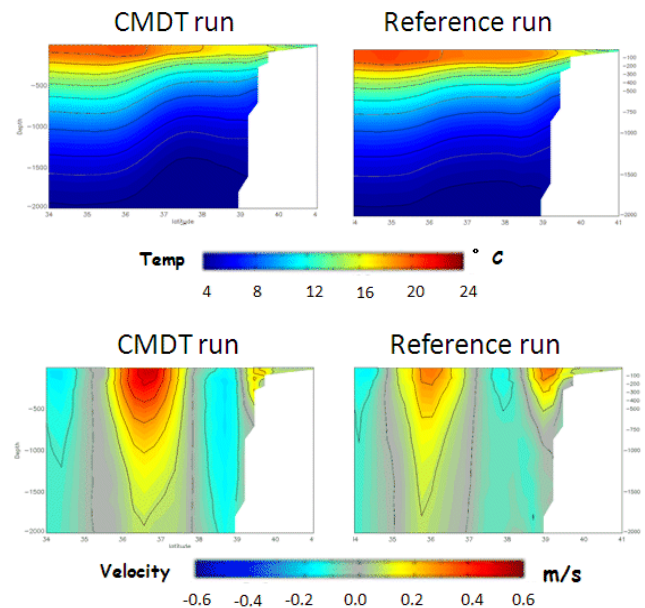
Fig. 5. Cross section of temperature (top) and zonal velocity (bottom) at 72^\circ W longitude in the Mercator CMDT run (left) and the reference run (right).
