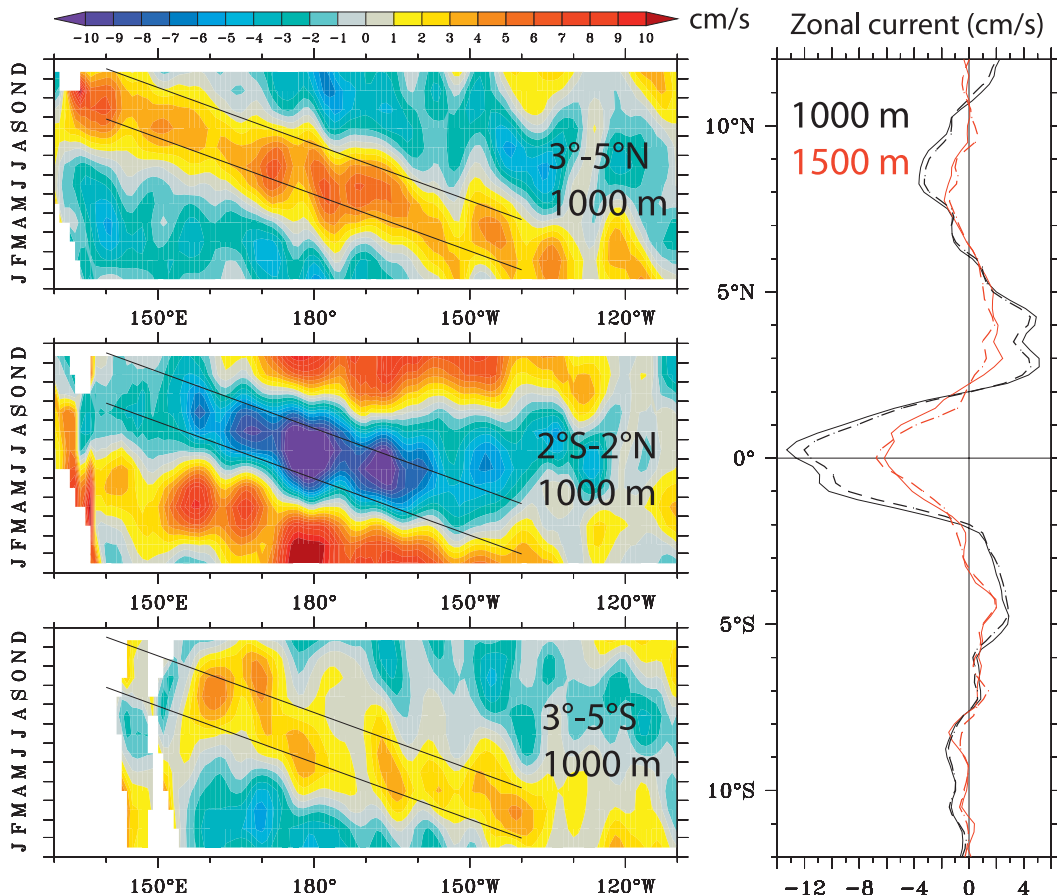
FIG. 6. (left) Seasonal anomalies (mean removed) of 1000-m zonal currents ( \text{cm s}^{-1} ) averaged between (top) 3^{\circ} – 5^{\circ}\text{N} , (middle) 2^{\circ}\text{S} – 2^{\circ}\text{N} , and (bottom) 3^{\circ} – 5^{\circ}\text{S} . (right) Zonal velocity anomalies averaged along the paths shown in the left panels (in black lines), between 160^{\circ}\text{E} and 160^{\circ}\text{W} , for 1000-m current anomalies (thin black) and their first annual harmonic (dashed black). The same calculations have been made for zonal current anomalies at 1500-m currents, and 1500-m zonal currents anomalies and their first annual harmonic have been averaged along similar Rossby paths, shifted one month in advance (red thin and dashed lines).
