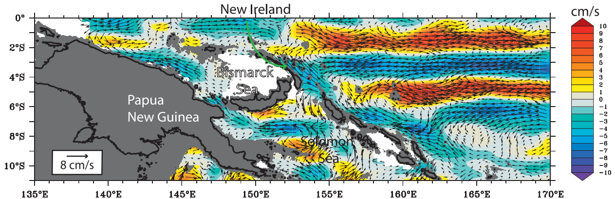
FIG. 5. Mean 1000-m zonal and meridional currents ( \text{cm s}^{-1} ; vectors) in the southwest tropical Pacific. Colors represent the mean zonal current (scale at right). Topography shallower than 1000-m depth is shaded in dark gray. White areas (as in Bismarck Sea) are locations with no data.
