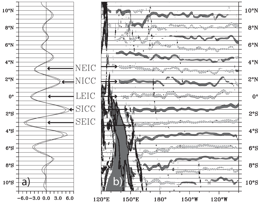
FIG. 3. (left) Mean zonal current u at 1000 m in \text{cm s}^{-1} , zonally averaged in the 160°E–120°W band in the Southern Hemisphere and in the 120°E–120°W band in the Northern Hemisphere. Thick lines are the gridded u , and thin lines are the reconstruction from CD. (right) Positions of the CD-reconstructed zonal jets. Eastward jets are in dark gray; westward jets are in light gray.
