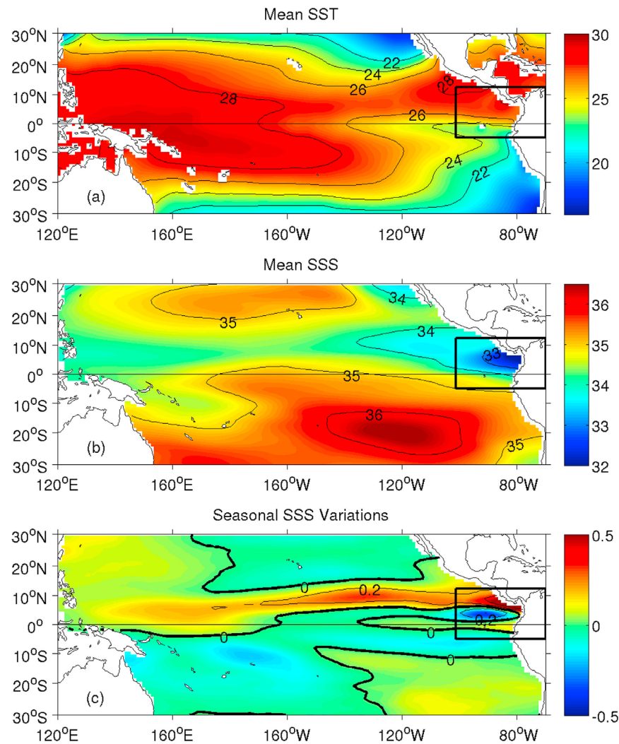
Figure 1. Mean (a) SST (°C), (b) SSS and (c) first seasonal EOF of SSS in the tropical Pacific Ocean. Seasonal values correspond to peak anomalies in March; opposite anomalies are found in October. The eastern box delimits our region of study.
