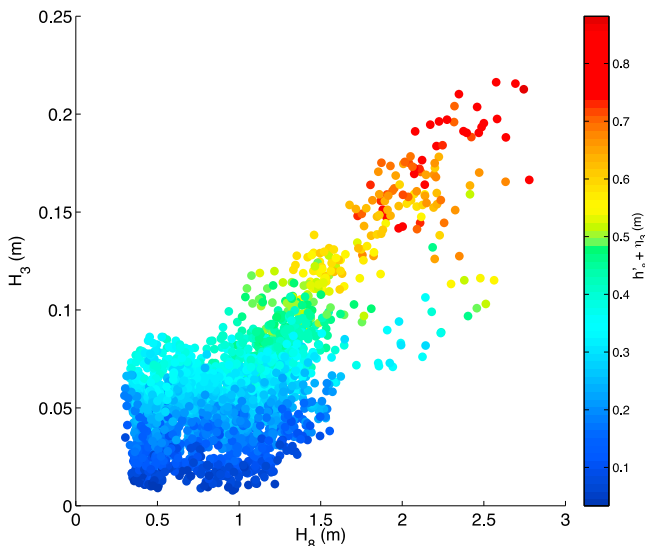
Figure 4. Water level effects on reef flat wave height. Reef flat rms wave height H_3 versus incident wave height H_8 , with color indicating the water depth at sensor 8 with the mean removed h_3' , plus the setup at sensor 3. Wave heights where \bar{h}_3 < 0.3 m are excluded.
