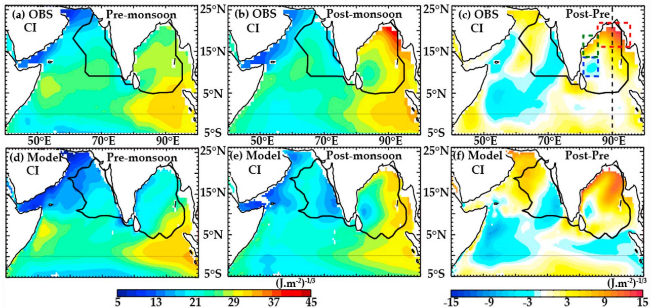
Figure 6. Climatological cooling inhibition index (CI; in (\text{J.m}^{-2})^{-1/3} ) for (a and d) premonsoon and (b and e) postmonsoon seasons, and (c and f) their difference using (top) observations and (bottom) the model over the 1978–2007 period. The thick contour delineates a region where 80% of TCs occur in the northern Indian Ocean (see Figure 1) while dashed colored boxes on Figure 6c are same as in Figure 3. The black dashed line indicates the temperature and salinity section at 90^{\circ}\text{E} shown on Figure 5.
