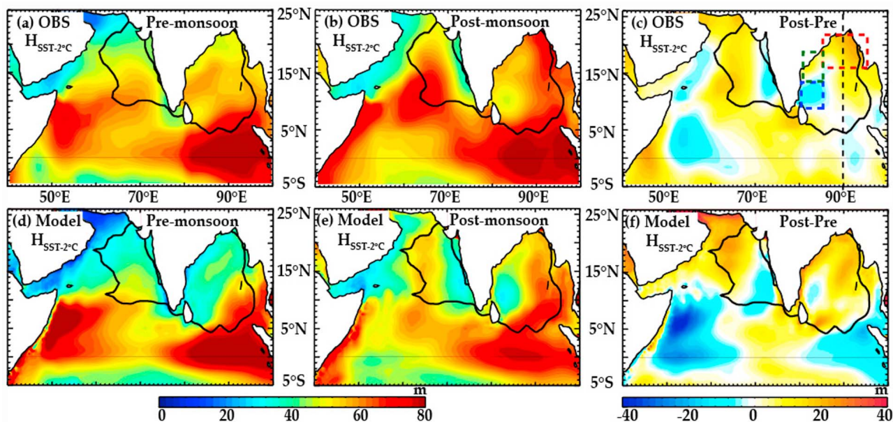
Figure 4. Climatological depth at which the ocean temperature is 2^{\circ}C below the surface temperature (in meters) for (a and d) premonsoon and (b and e) postmonsoon seasons, and (c and f) their difference derived from (top) de Boyer Montégut et al. [2004] climatology and (bottom) the model over the 1978–2007 period. The thick contour delineates a region where 80% of TCs occur in the northern Indian Ocean (see Figure 1) while dashed colored boxes on Figure 4c are same as in Figure 3. The black dashed line indicates the temperature and salinity section at 90^{\circ}E shown on Figure 5.
