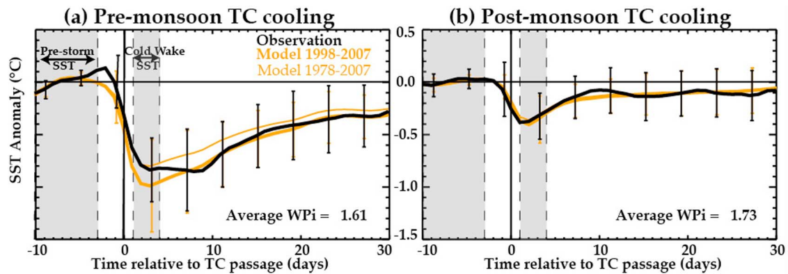
Figure 7. Composite evolution of TC-induced SST cooling within 200 km of TC-tracks in the BoB (in °C) during (a) premonsoon and (b) postmonsoon seasons for observations (black line) and the model over the 1998–2007 period (thick orange line) and the model over the 1978–2007 period (thin orange line). Vertical bars (black for the observations and orange for the model) indicate the spread around the mean, evaluated from the lower and upper quartiles. These quartiles are not shown for the model results over the 1978–2007 period for clarity.
