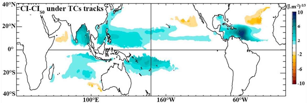
Figure 15. Spatial distribution of the difference between average standard CI underneath TC tracks (in (\text{J.m}^{-2})^{-1/3} ) minus \text{CI}_{50} calculated over the 1978–2007 period. Both quantities are estimated from the weekly averaged stratification model outputs, within 200 km and between 10 days and 3 days before each cyclone eye passage location. This plot indicates where salinity stratification inhibits (blue shades) or enhances (red shades) TC-induced cooling.
