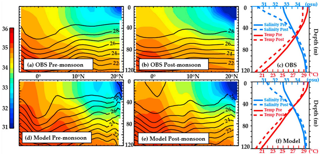
Figure 5. Latitude-depth section (at 90^{\circ}\text{E} ) of observed climatological salinity (in psu; color) and temperature (in ^{\circ}\text{C} ; contour) in the BoB during (a) premonsoon and (b) postmonsoon seasons. (c) Observed temperature (red) and salinity (blue) profiles averaged in the BoB north of 15^{\circ}\text{N} for premonsoon (plain line) and postmonsoon (dashed line) seasons. (d–f) Same for model outputs over 1978–2007.
