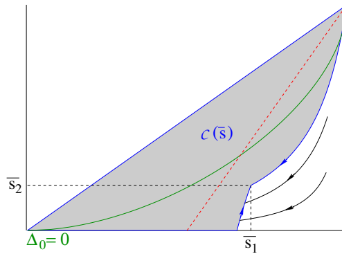
Figure 6: Optimal trajectories for a target \bar{s} \in \Delta_{SA}^- such that \Delta_{SA} \not\subset \mathcal{C}(\bar{s}) . Picture left: \bar{s} \in \mathcal{R}^- \cap \Delta_0^+ . Picture right: \bar{s} \in \mathcal{R}^- \cap \Delta_0^-
