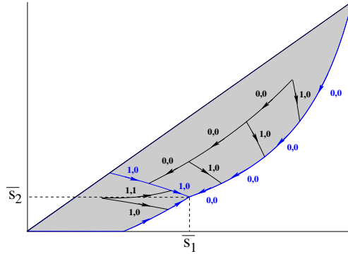
Figure 3: In the case where an initial condition s_0 is in \mathcal{C}(\bar{s}) with \bar{s} = (1, 0.3) , there exist infinitely many trajectories steering s_0 to \bar{s} in time v(s_0) , where v is given by (3.2). When s_0 is below the curve \Gamma , the control u_1 is always equal to 1 whereas if s_0 is above \Gamma , then the control u_2 is always equal to 0.
