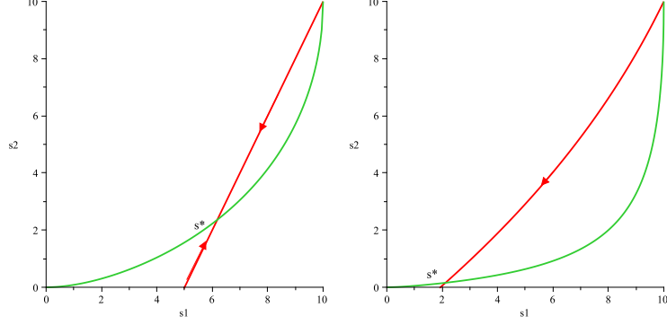
Figure 4: Picture left: plot of the singular arc \Delta_{SA} (in red) and of \Delta_0 (in green) in the linear case: \mu(s) = s , s_{in} = 10 . Picture right: plot of the singular arc \Delta_{SA} (in red) and of \Delta_0 (in green) in the Monod case: \mu(s) = \frac{s}{5+s} , s_{in} = 10 .
