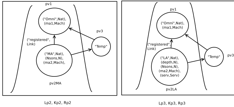
Fig. 3. Addition of a non-terminal term
