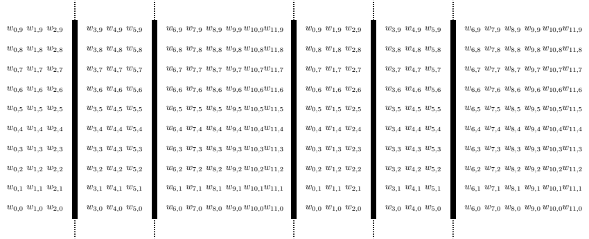
FIGURE 4. A periodic point of A . Here w_{i,j} are symbols of the alphabet of W .
