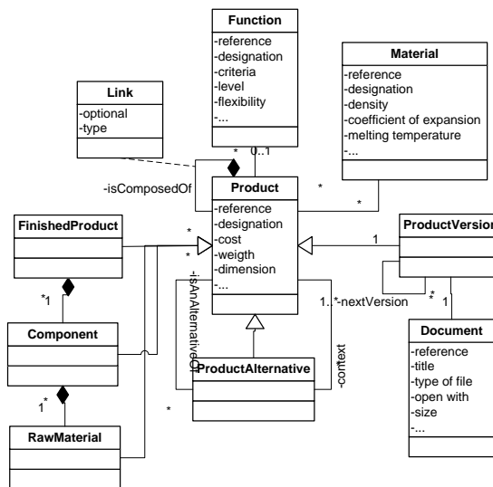
Figure 2: Product class diagram.
