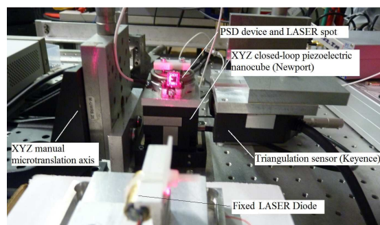
Figure 2. The experimental PSD setup in direct laser spot mode.
