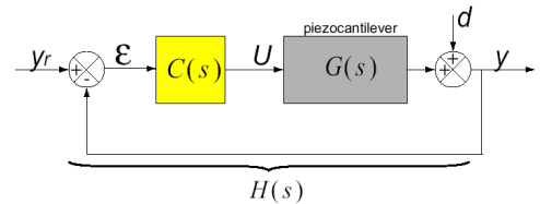
Fig. 13. Block-scheme of the closed-loop.
