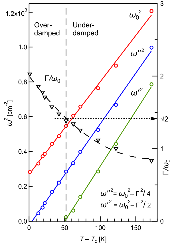
FIG. 3: (color online) Temperature evolution of soft mode spectral parameters in paraelectric phase of \text{PbTiO}_3 . Temperature dependence of the soft mode frequency squared ( \omega_0^2 ) was adjusted to a linear (Cochran) law discussed in the text (full line). The quantities \omega''^2 and \omega'^2 show analogical behavior. The vertical lines indicated crossover between over-damped and underdamped soft mode regime. Triangle symbols stand for the relative soft mode damping - the ratio of damping and soft mode frequency \Gamma/\omega_0 . These data correspond to the right-hand side scale.
