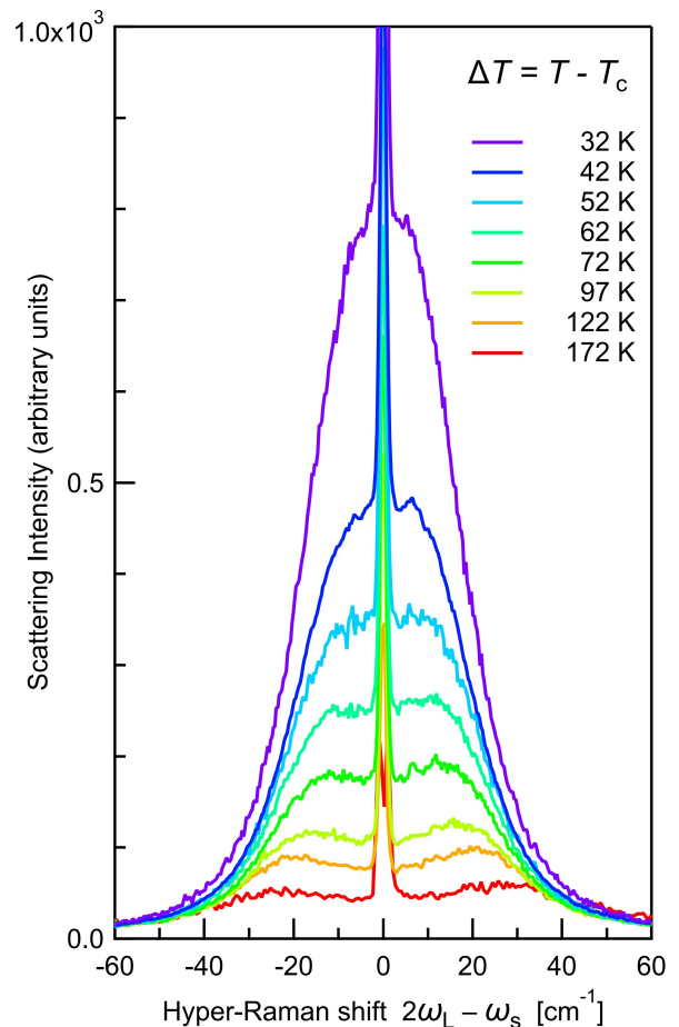
FIG. 1: (color online) Unpolarized (V+H) HRS spectra of in paraelectric phase of \text{PbTiO}_3 single crystal for several temperatures indicated in the figure with respect to the phase transition ( T_C \approx 760 \text{ K} ). These spectra are not corrected for temperature factor.
