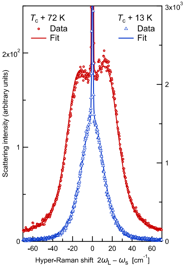
FIG. 2: (color online) Unpolarized (V+H) HRS spectra of PMN at 13 K and 72 K above the phase transition ( T_C \approx 760 K) adjusted to the model of DHO. The resolution limited central line is adjusted by a narrow Gaussian peak.
