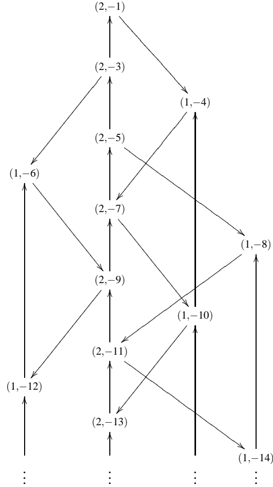
Figure 7: The quiver \Gamma^- for \mathfrak{g} of type G_2 .
