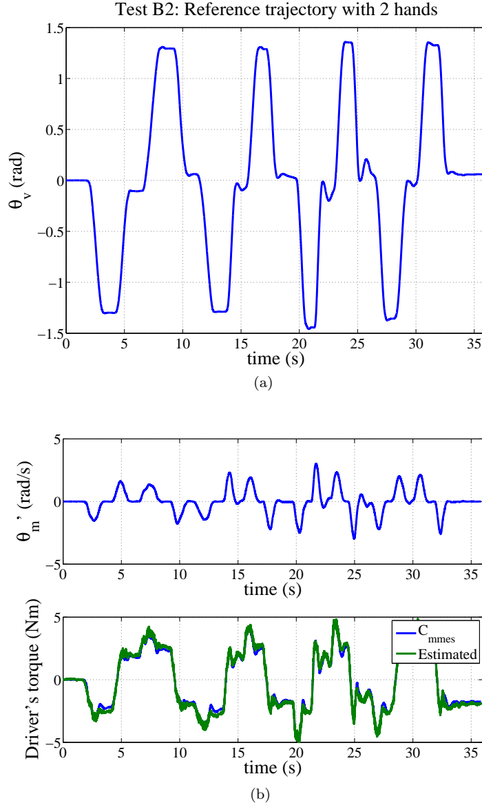
Figure 11: Observer validation: (a) Trajectory imposed on the test, with two hands and oscillation annealing control. (b) Profile of the angular speed of the electrical motor and comparison of the estimated torque with the driver's torque measure C_{mmeas}
