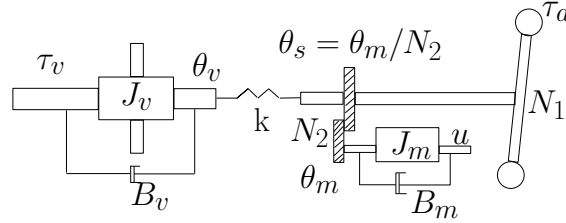
Figure 4: Mechanical model of the EPS system
