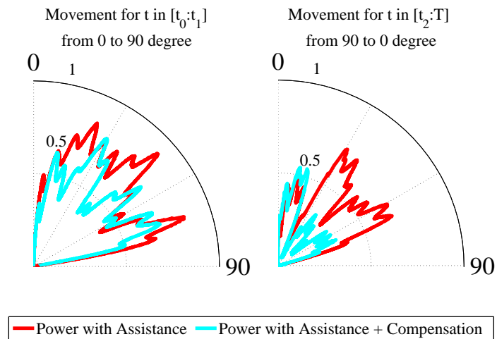
Figure 19: Power consumption during the experimental test
