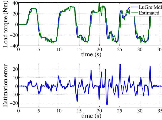
Figure 12: From the top to the bottom: comparison of the estimated torque with the load torque, obtained from the LuGre model, and estimation error.
