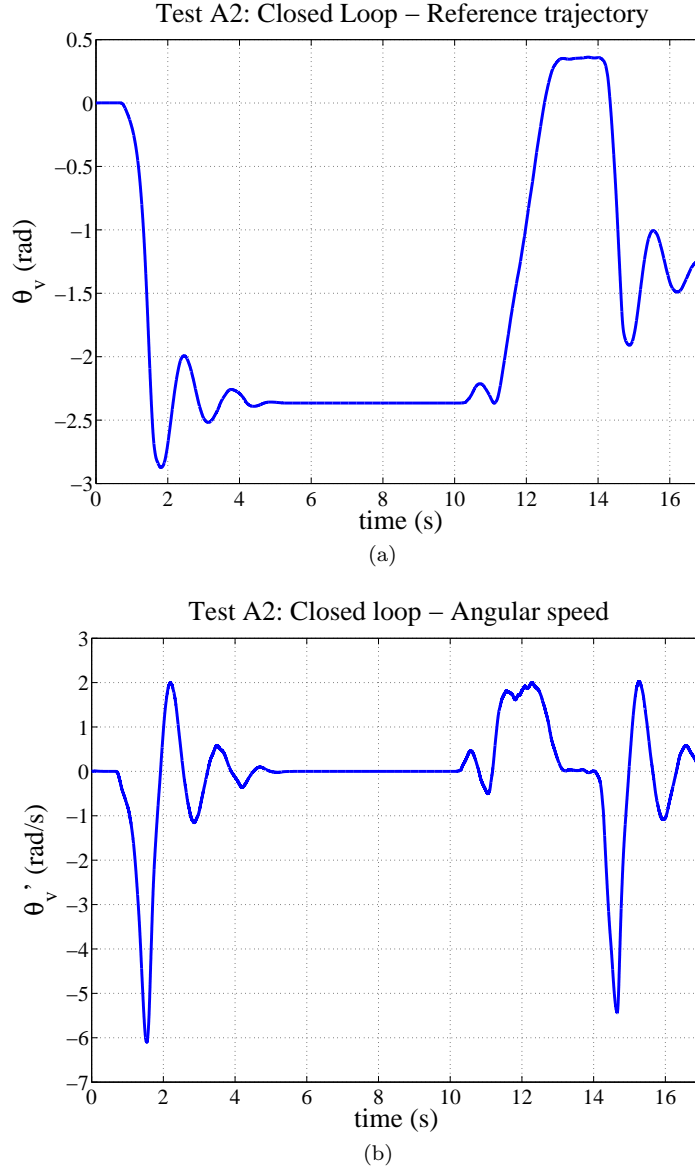
Figure 10: Angular position (a) and angular speed (b) of the steering wheel. The oscillations of the steering column are annealed by the LQR control.
