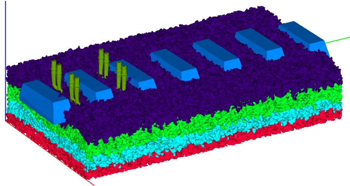
Figure 2: Tamping process on a railway slice of seven sleepers
