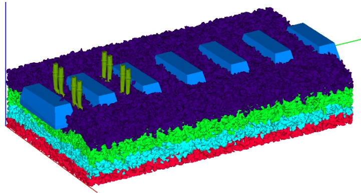
Figure 2: Tamping process on a railway slice of seven sleepers
