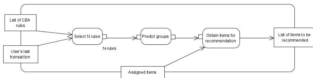
Figure 3. Runtime process
