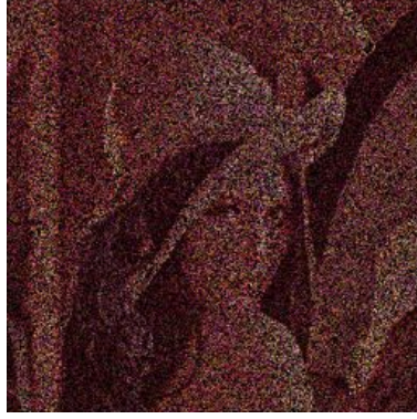
(b) PSNR=6.883
