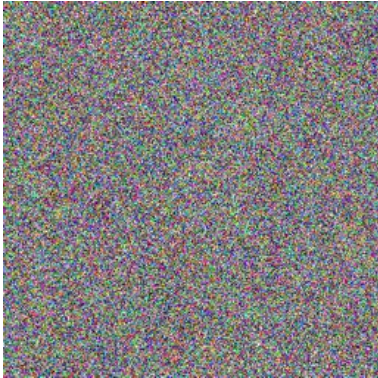
(g) PSNR=5.399
