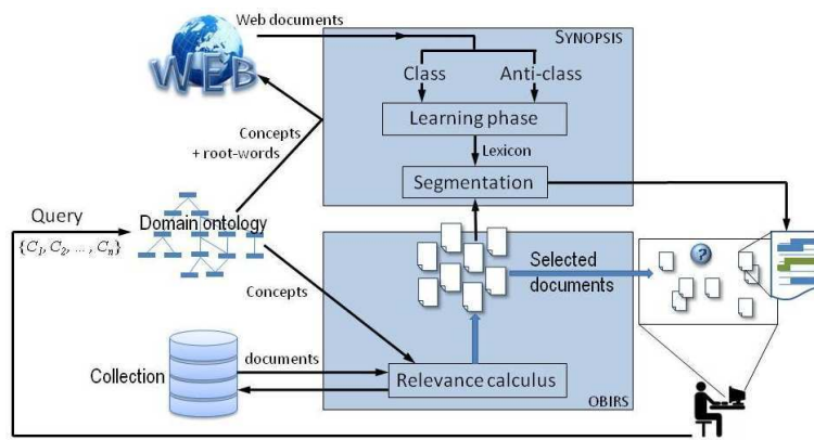
Fig. 1 Overview of our CoLexIR approach
