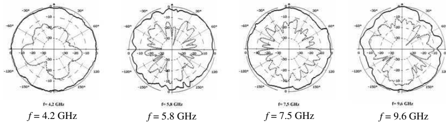
Figure 6. Radiation patterns of the planar monopole with fractal contour in the xy -plane at resonant frequencies 4.2, 5.8, 7.5, and 9.6 GHz. — E_\theta , - - - E_\phi .
