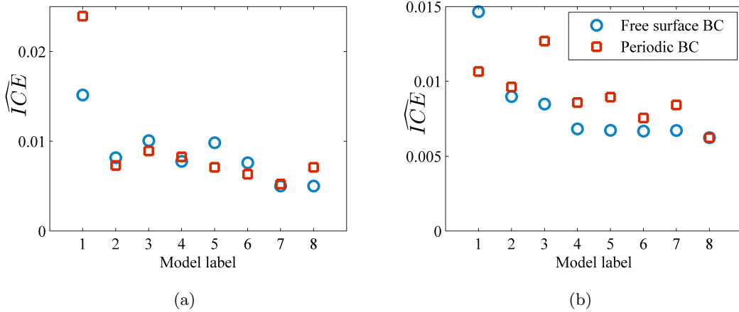
Figure 6: Variation of \widehat{ICE} of different assumed mixture models for computational cells consisting of (a) 125 grains and (b) 1000 grains.
