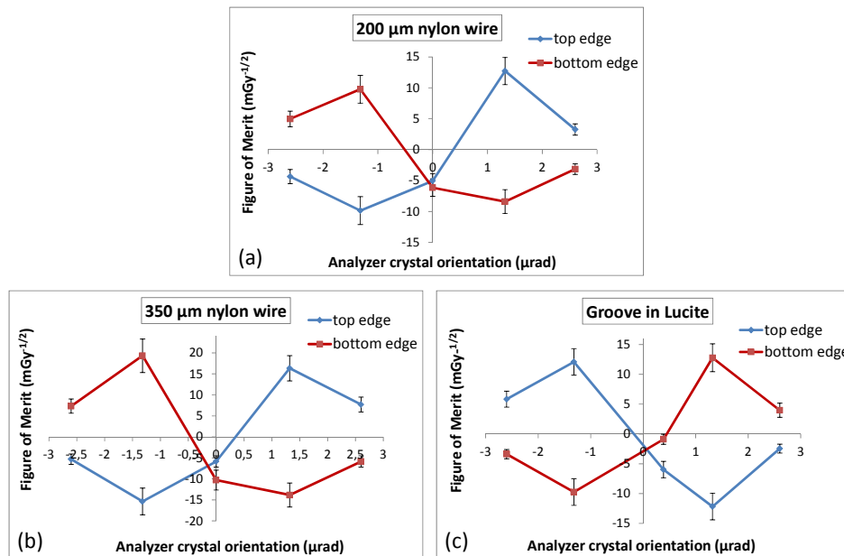
Fig. 6. Calculated values of the figure of merit (FoM) of the ABI edge signal for three different objects: (a) the 200 \mu\text{m} diameter nylon wire, (b) the 350 \mu\text{m} diameter nylon wire, (c) the groove in Lucite. Values at both the top and bottom edges are reported. The zero on the x axis corresponds to the Bragg condition (top) for the analyzer crystal.
