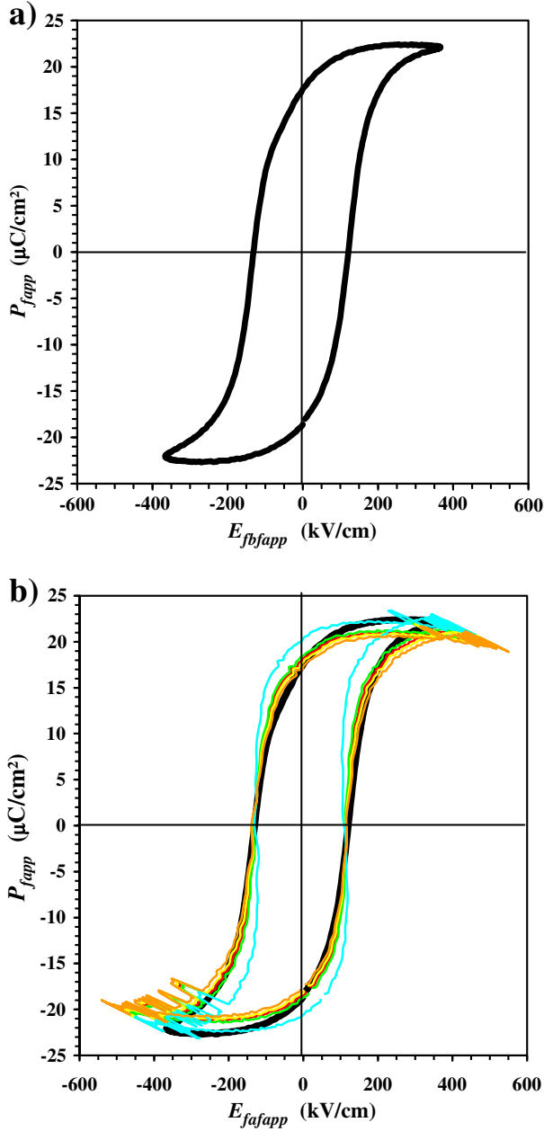
Fig. 5. a) Apparent polarization loop calculated from hysteresis measurement performed on the 400 nm thick PZT capacitor before fatigue (see the plot in thin black line on Fig. 1.a)). b) Polarization loop in thick black line is the same plot as a), colored loops are calculated from hysteresis measurement performed after fatigue (loop in thick red line on Fig. 1.b)). Clockwise rotational shift is observed when \Delta C_i is over estimated, counter clockwise rotational shift otherwise. The best fit was obtained for \Delta C_i = 1.4 nF.
