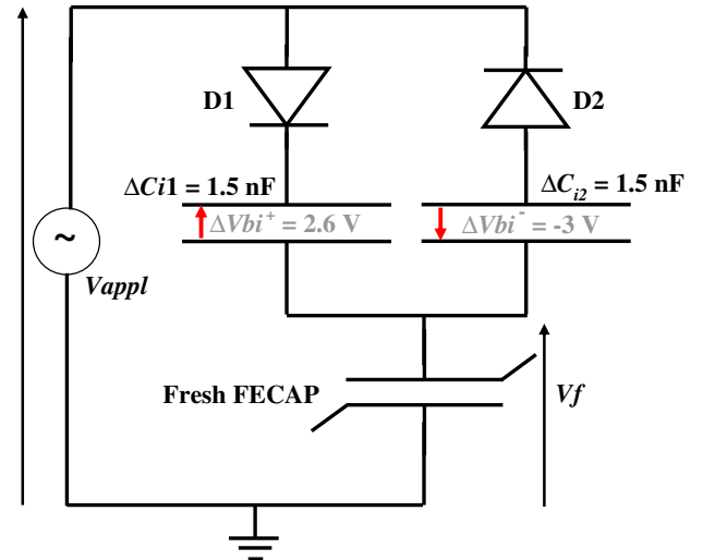
Fig. 7. Enhanced circuit used for the correct duplication of the screening effects caused by accumulation of charge at the interfaces and of the sign switching of this charge.
