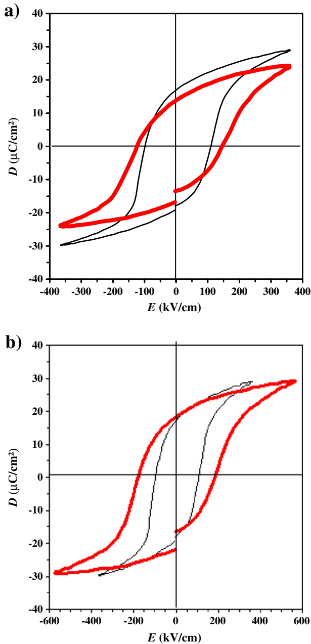
Fig. 8. a) Hysteresis loops of 400 nm thick PZT capacitor before fatigue (thin black line) and after using the circuit in Fig. 7 (thick red line), for same input voltage. b) Same plot as a) except that the voltage applied to the artificially fatigued capacitor was adjusted to achieve the same maximum electric displacement. This artificial fatigue must be compared with actual fatigue presented in Fig. 1.
