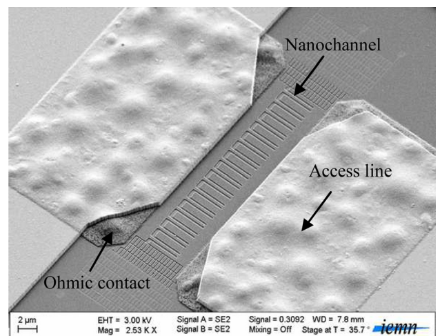
FIG. 2. SEM view of an array of 16 nanochannels.
