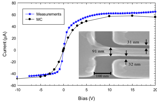
FIG. 3. Comparison of the measured I-V curve (blue stars) with the one obtained with MC simulation (black circles) corresponding to the device shown in the inset (SEM view: the length and width of the channel are about 1\ \mu\text{m} and 90\ \text{nm} , respectively).
