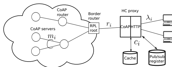
Figure 1: Scheme of the implemented caching system.
