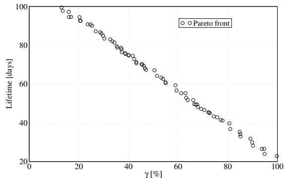
Figure 4: Pareto front of the considered caching architecture.
