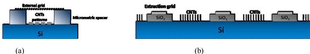
Fig. 5 External grid (a) and integrated-grid (b) cathode
