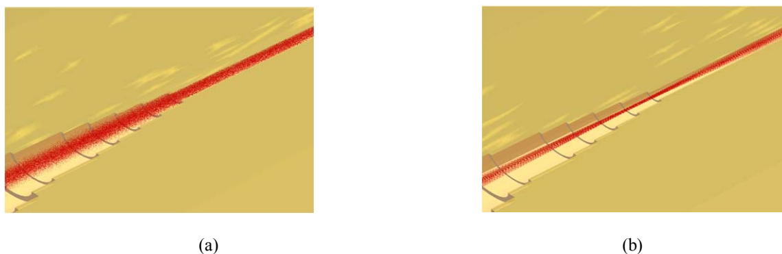
Fig. 4 Effect of transverse velocity on the focusing: an electron beam propagating in the electron gun anode (a) without transverse velocity, (b) with transverse velocity
