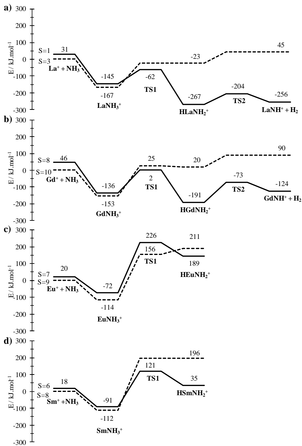
Figure 4. Energy profiles for reactions of \text{NH}_3 on \text{Ln}^+ in low (—) and high (---) spin multiplicities relative to \text{Ln}^+ (High spin) + \text{NH}_3 , including ZPE calculated at the B3LYP level.
