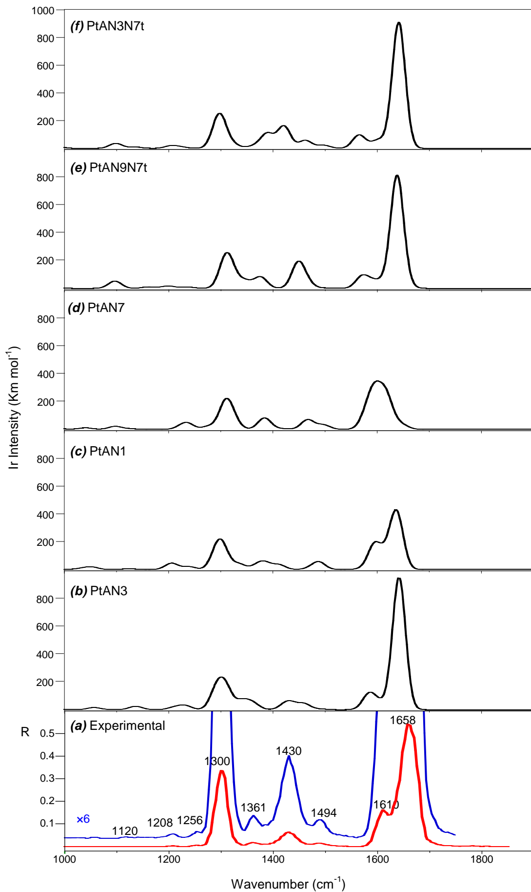
Figure 6. a) Experimental IRMPD spectrum of cis\text{-}[\text{Pt}(\text{NH}_3)_2(\text{A})\text{Cl}]^+ together with computed IR spectra of b) PtAN3, c) PtAN1, d) PtAN7, e) PtAN9N7t and f) PtAN3N7t, all calculated at the at the B3LYP/ 6-311G** level, in the spectral range of 1000-1900 \text{cm}^{-1}
