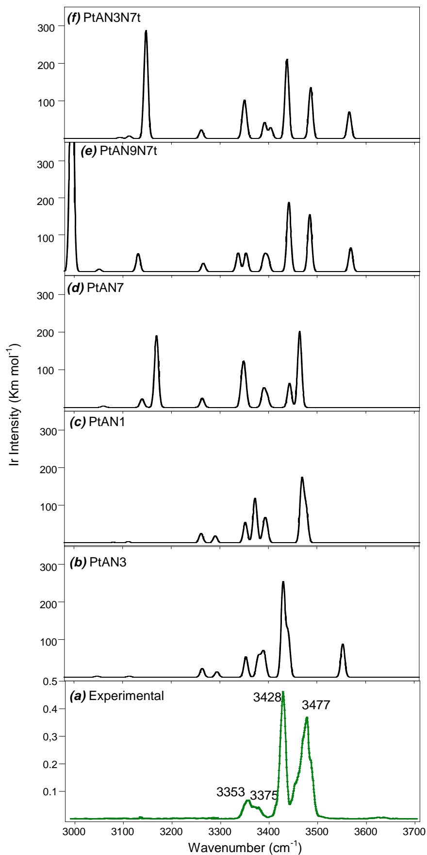
Figure 7. a) Experimental IRMPD spectrum of cis -[Pt(NH 3 ) 2 (A)Cl] + together with computed IR spectra of b) PtAN3, c) PtAN1, d) PtAN7, e) PtAN9N7t and f) PtAN3N7t, all calculated at the at the B3LYP/ 6-311G** level, in the spectral range of 3000-3700 cm -1 .
