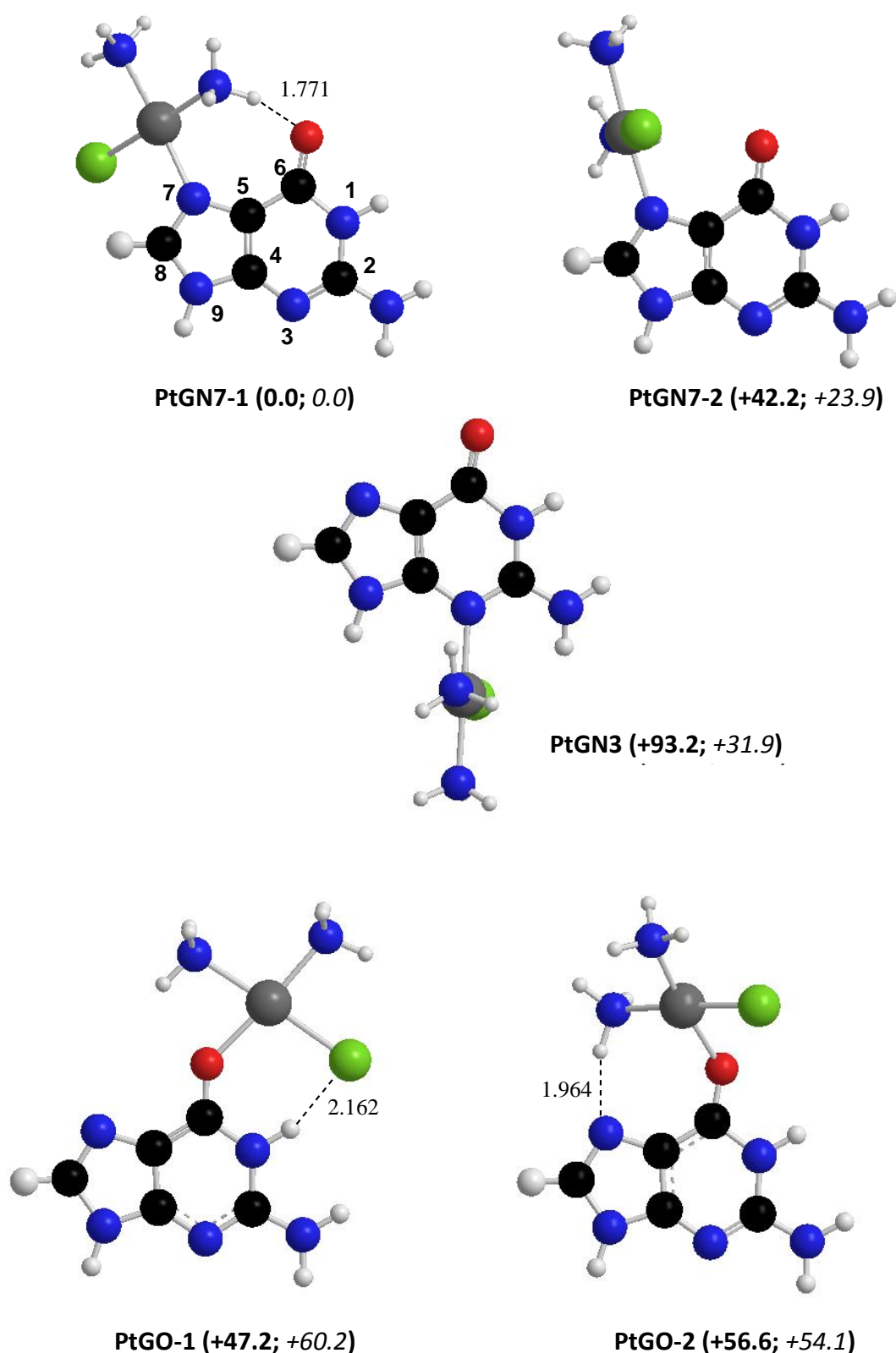
Figure 2. Geometries and relative free energies ( \text{kJ mol}^{-1} , in parentheses) for representative cis - [\text{Pt}(\text{NH}_3)_2(\text{G})\text{Cl}]^+ structures calculated at the B3LYP/6-311G** level. Distances are given in Angströms. Relative free energies given in italics were obtained by using the Polarized Continuum Model (PCM) approach
