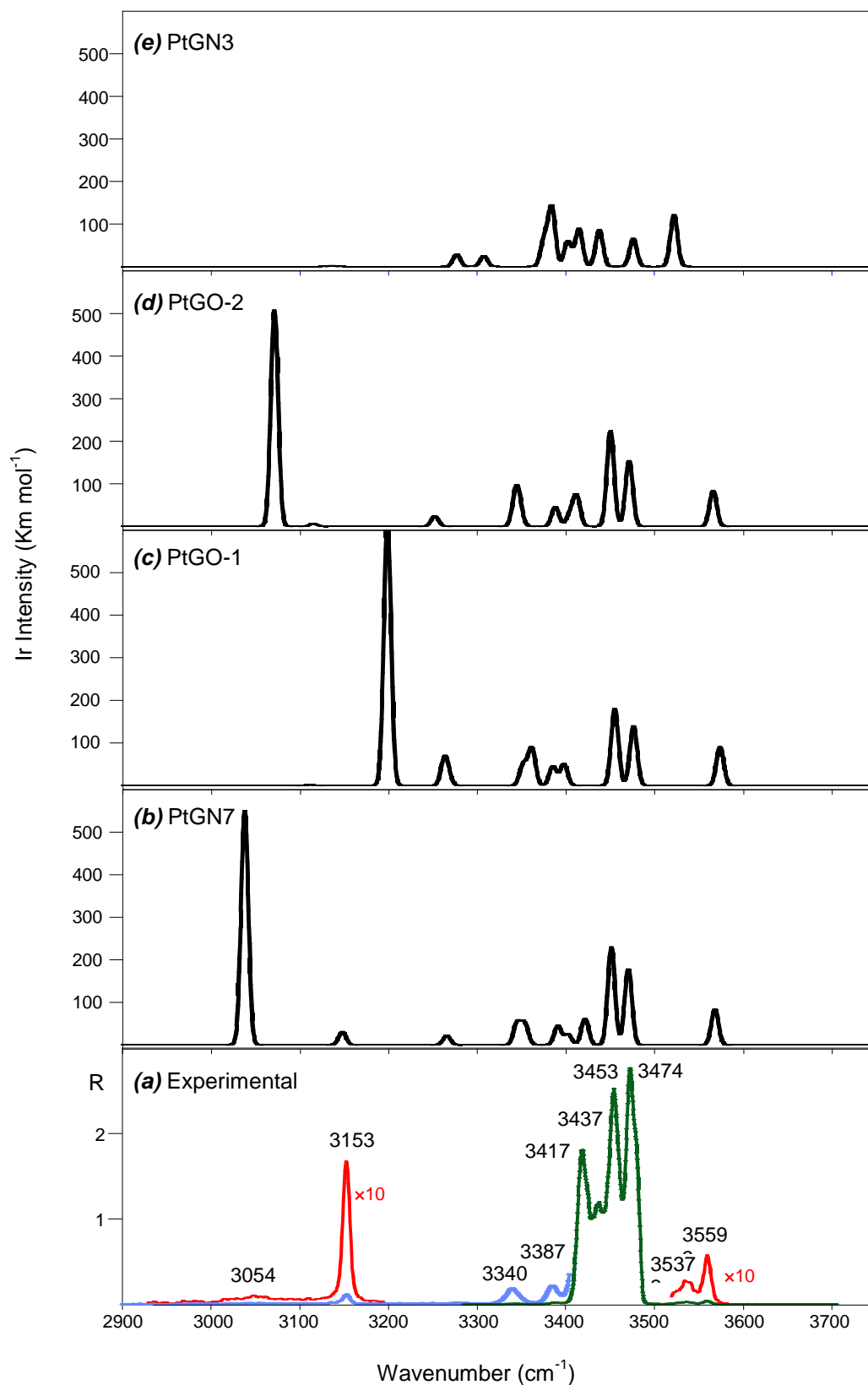
Figure 4. a ) Experimental IRMPD spectrum of cis\text{-}[\text{Pt}(\text{NH}_3)_2(\text{G})\text{Cl}]^+ obtained with an irradiation time of 1 second (green) and 2 second (blue) respectively, together with computed IR spectra of b ) PtGN7-1, c ) PTGO-1, d ) PtGO-2 and e ) PtGN3, all calculated at the B3LYP/ 6-311G** level in the spectral range of 2900-3700 \text{cm}^{-1} .
