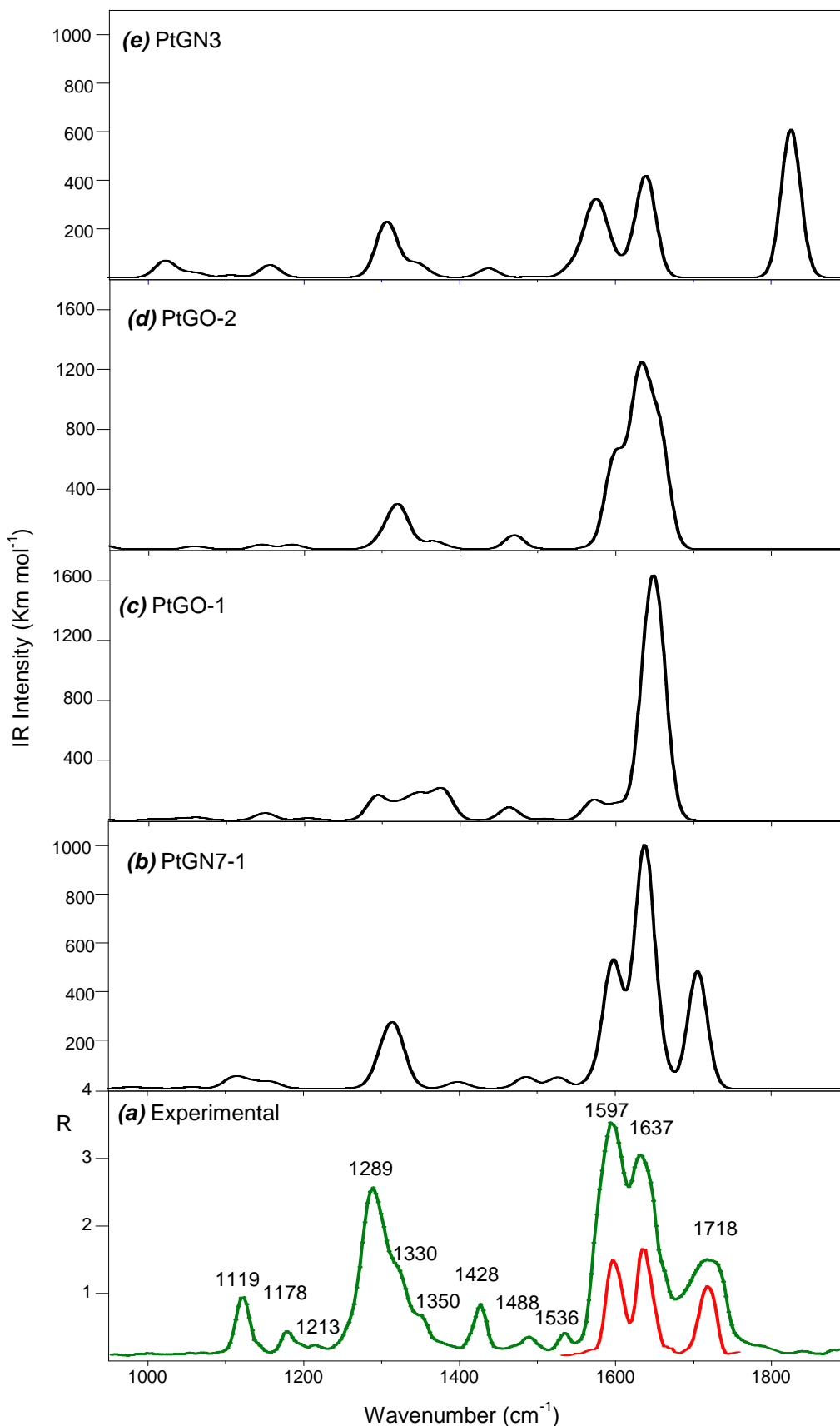
Figure 3. a ) Experimental IRMPD spectrum of cis\text{-}[\text{Pt}(\text{NH}_3)_2(\text{G})\text{Cl}]^+ obtained with full (green) and attenuated (by a factor of two, red) laser power together with computed IR spectra of b ) PtGN7-1 c ) PtGO-1, d ) PtGO-2 and e ) PtGN3, all calculated at the B3LYP/ 6-311G** level in the spectral range of 950-1900 \text{cm}^{-1} .
