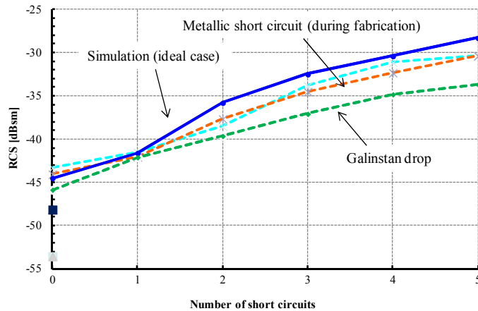
Fig. 8 : RCS of antenna array with different number of short circuits
