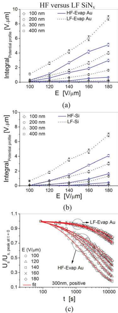
Fig. 10. The influence of the dielectric deposition conditions: the integral of the surface potential profile as a function of the applied electric field intensity, E , for SiN x films deposited using the HF and LF recipes with different film thicknesses over (a) evaporated Au layers and (b) directly over silicon substrates; (c) the surface potential decay for the HF-Evap Au and LF-Evap Au samples with 300 nm film thicknesses, for charges which have been injected under different electric field intensities, E .
