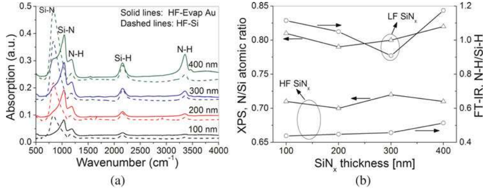
Fig. 3. Physical material characterization for different samples: (a) FT-IR spectra of HF-Evap Au and HF-Si \text{SiN}_x films with different thicknesses, and (b) the N/Si ratio from XPS and the N-H/Si-H ratio from FT-IR for HF and LF materials.
