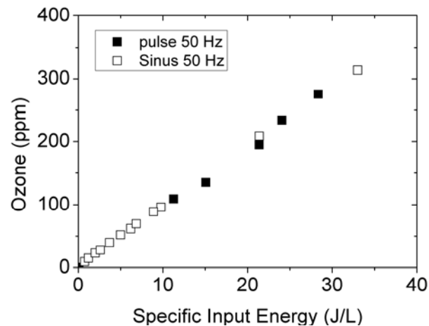
Figure 14. Ozone concentration measured downstream of the reactor vs. specific input energy for the pin-to-pin reactor (68 pins) energized by a 50Hz ac power supply and the pulsed power supply; dry air 1L/min.
