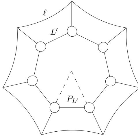
FIGURE 4. The 7-holed heptagon
