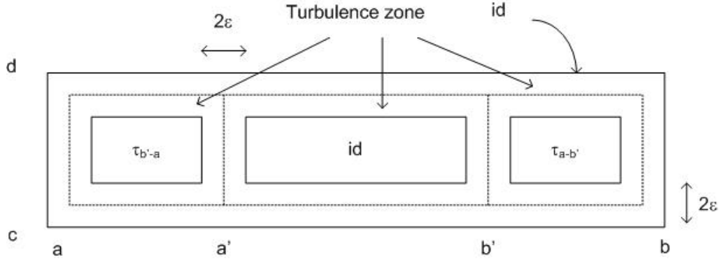
Figure 3: A quasi-permutation: it permutes the two lateral boxes, and keeps the central one fixed.
