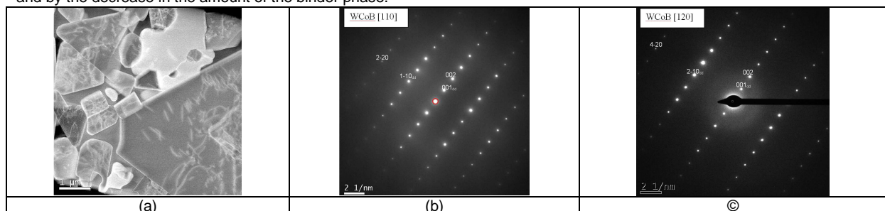
Fig. 11. TEM observation of a WCoB phase (lighter phase) in a WC-Co substrate (a), diffraction of the WCoB phase on [110] (b), diffraction of the WCoB phase on [120] (c)
