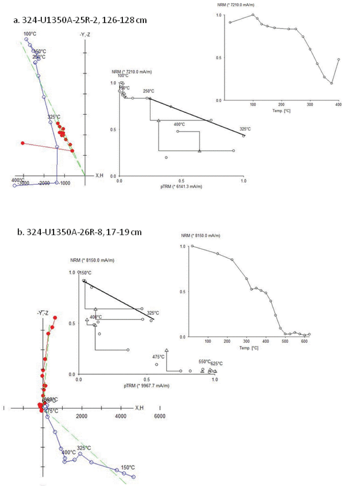
Figure 9. Examples of Arai plots, Zijdeveld diagrams and demagnetization spectra for two samples from Hole U1350A that did not give a reliable palaeointensity estimate. (a) Sample 324-U1350A-25R-2, 126–128 cm; (b) Sample 324-U1350A-26R-8, 17–19 cm.
