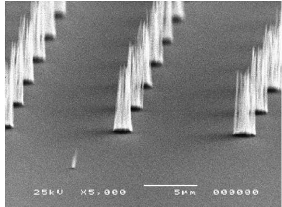
Fig. 4. SEM micrograph (with an enlarged view) of an array of aligned MWCNTs on Ni dots ( 1.6 \mu\text{m} in diameter) realized by optical lithography. The dot pitch is 10 \mu\text{m} .
