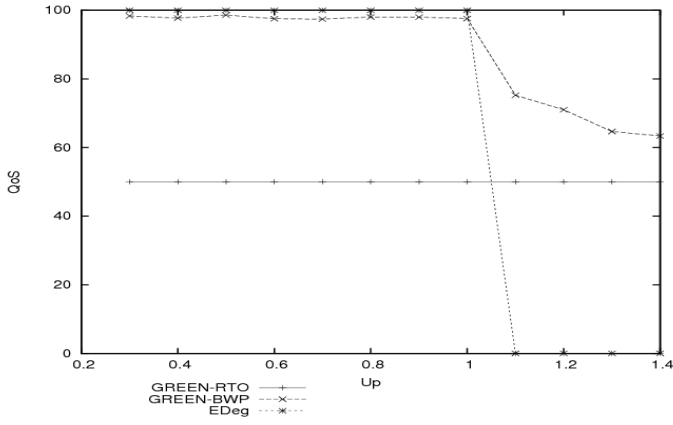
Fig. 2. QoS Performance comparison ( R_e = 1 and s_i = 2 )
