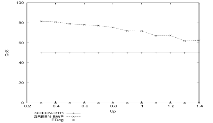
Fig. 5. QoS Performance comparison ( E(0) = \frac{P * P_r}{10} )
