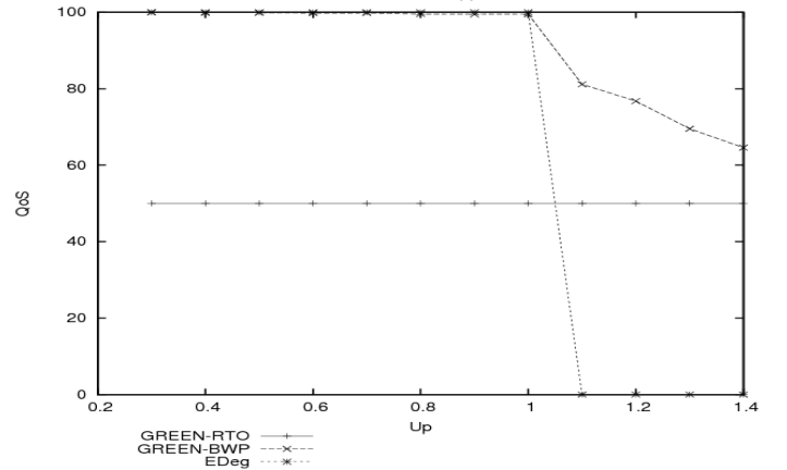
Fig. 4. QoS Performance comparison ( E(0) = P * P_r )
