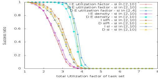
Fig. 1. EDF-based sorting criteria with WF heuristic
