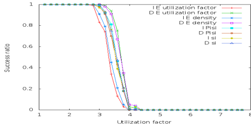
Fig. 2. EDF-based sorting criteria with FF heuristic with s_i in [2, 10]
